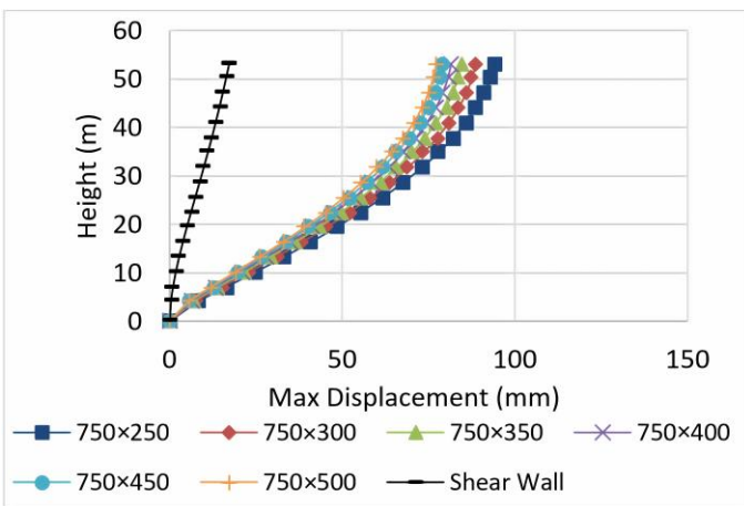
a) X-direction (b) Y-direction Fig. 10: Influence of column size on the maximum displacement of RC framed buildings
