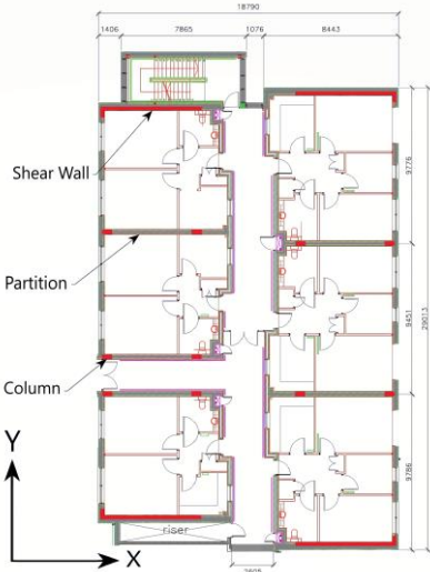
a) Architectural plan (values in mm)
