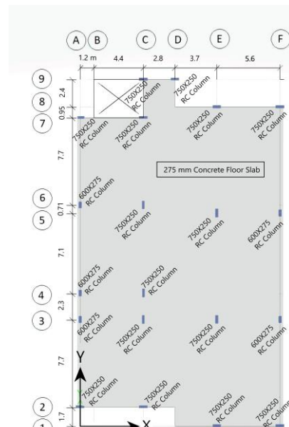
b) Modified plan design
