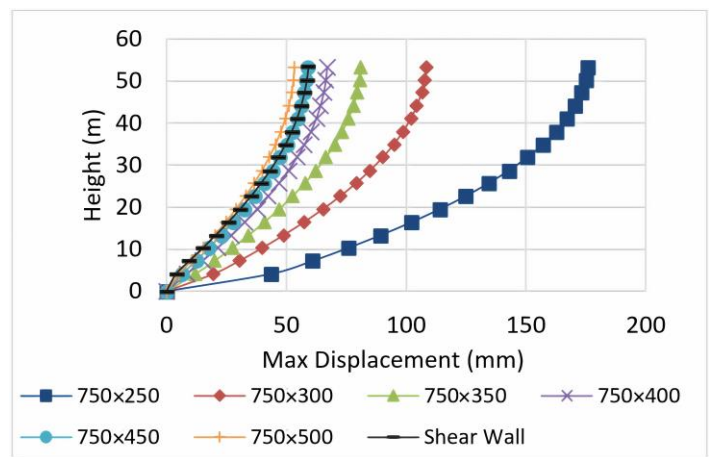
a) X-direction (b) Y-direction Fig. 10: Influence of column size on the maximum displacement of RC framed buildings
