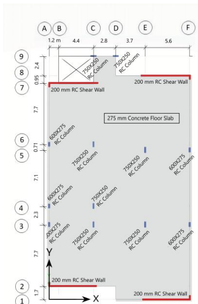
a) Reference plan design
