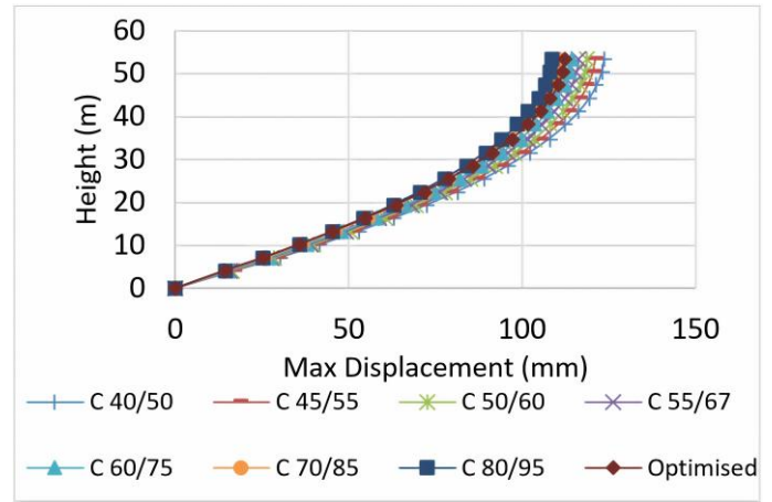
(a) -direction (b) Y-direction Fig. 9: Influence of concrete strength on the maximum displacement of RC framed buildings
