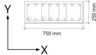
Fig. 8: Column cross-section
