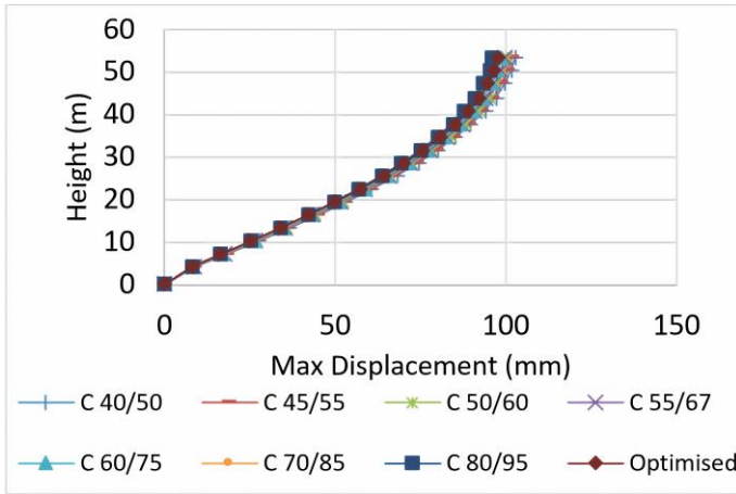
(a) -direction (b) Y-direction Fig. 9: Influence of concrete strength on the maximum displacement of RC framed buildings
